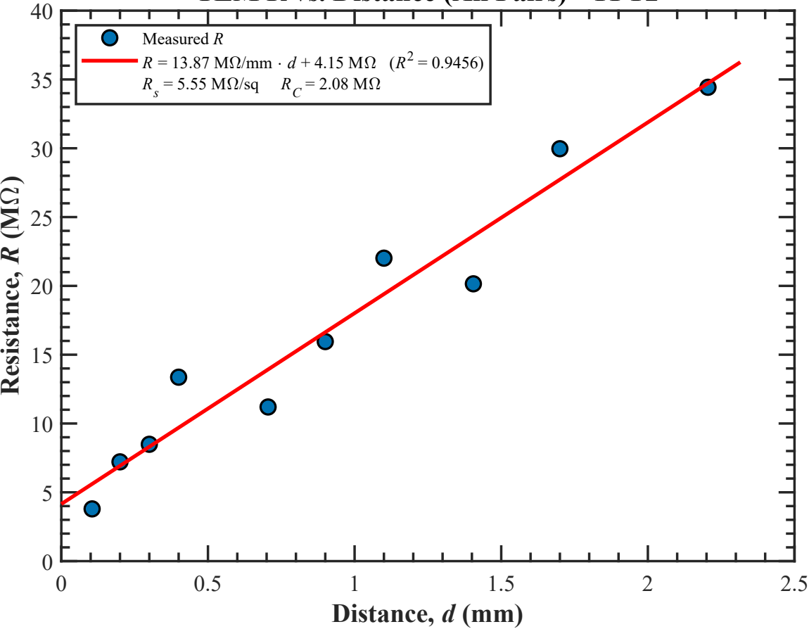
TLM R vs. Distance (All Pairs) - TFT2
